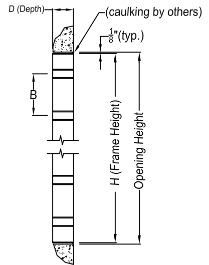
VERTICAL SECTION
