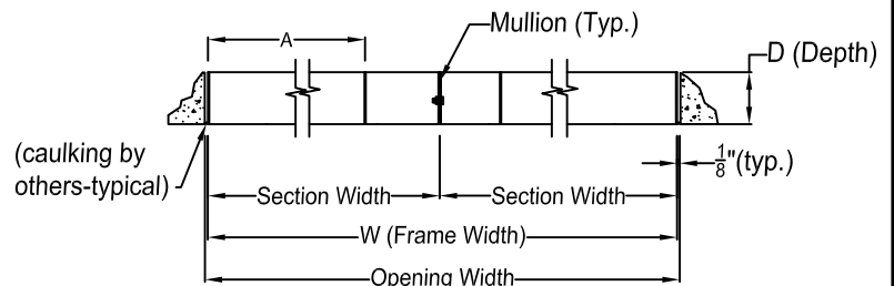
HORIZONTAL SECTION
