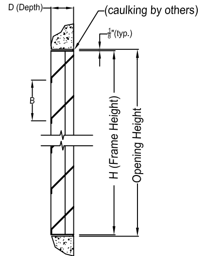
VERTICAL SECTION
