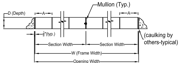
HORIZONTAL SECTION
