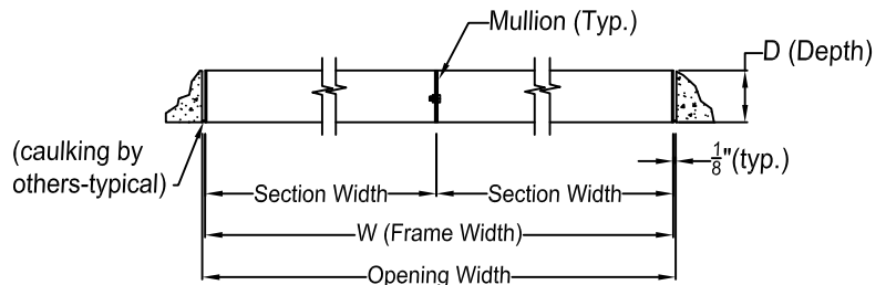
HORIZONTAL SECTION
