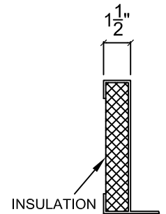
SECTION "A-A" UMB-8 INSULATED
