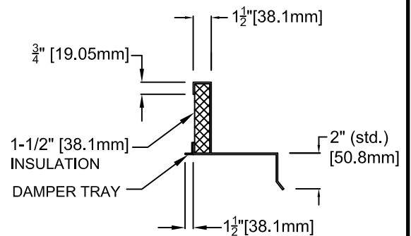
FCA-1 SECTION VIEW
