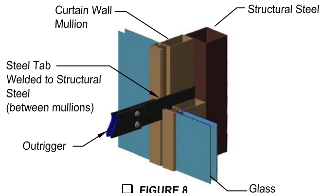
FIGURE 8 Steel Bracket Welded to Steel Support Behind Curtain Wall
