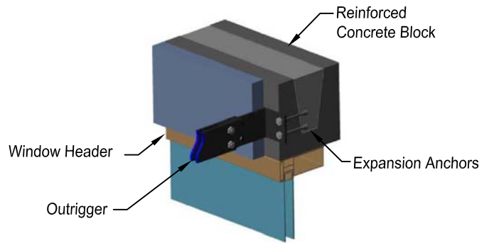
FIGURE 4 Bolted to Concrete Lintel
