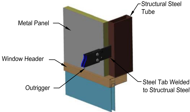
FIGURE 3 Steel Bracket Welded to Steel Support
