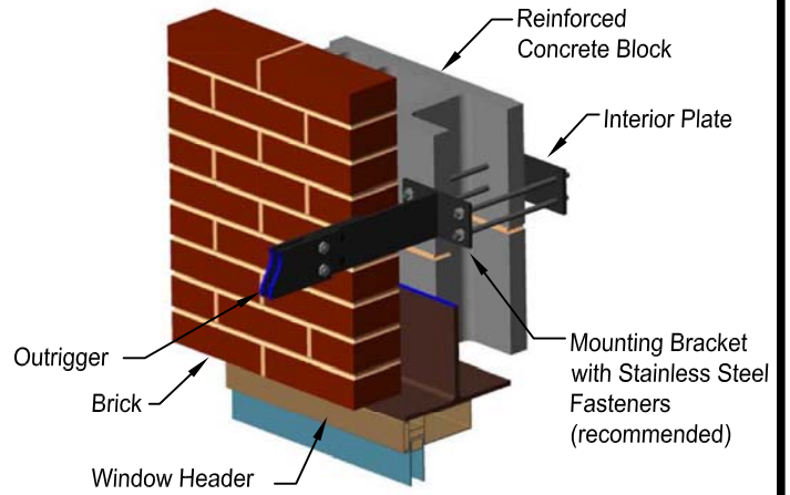
FIGURE 2 Through Bolted to Block
