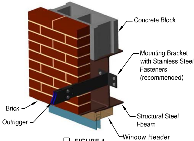
FIGURE 1 Bolted to Steel
