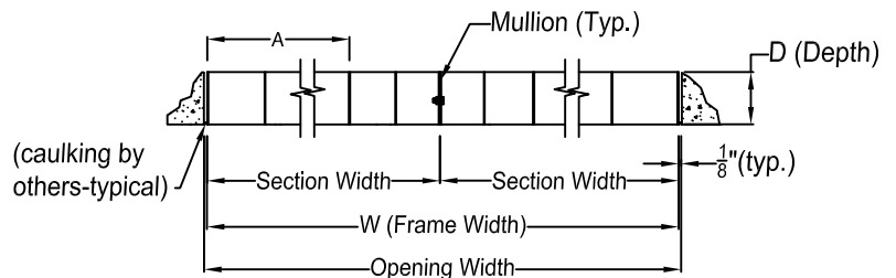
HORIZONTAL SECTION
