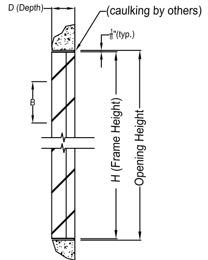
VERTICAL SECTION
