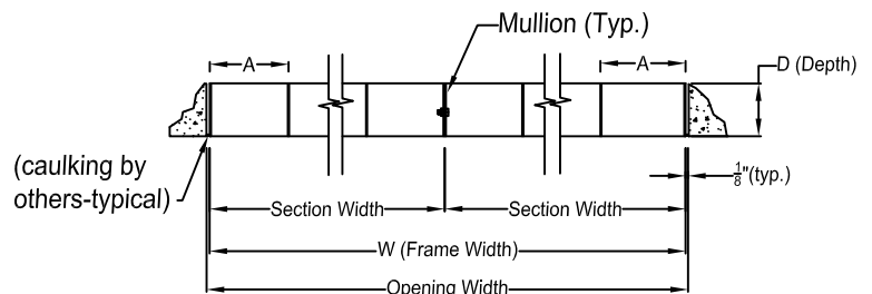
HORIZONTAL SECTION
