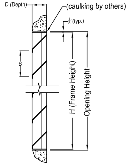
VERTICAL SECTION
