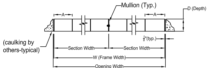
HORIZONTAL SECTION
