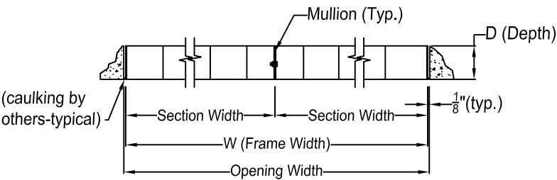
HORIZONTAL SECTION
