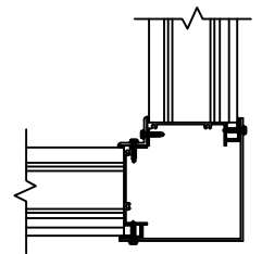
Mitered Corner Detail (Optional)
