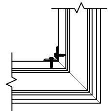
Mitered Corner Detail (Optional)
